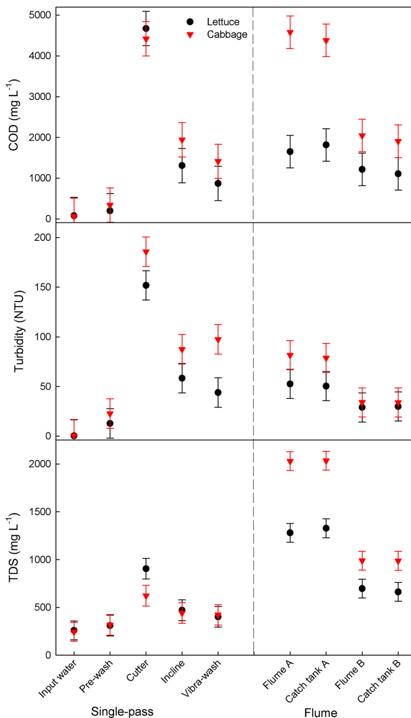
Fig. 2. Chemical oxygen demand (COD), turbidity, and total dissolved solids (TDS) of wash water samples were averaged across all time points during 2.7 h of production with estimated standard error. Flume system data from Luo et al. (2018) are shown for comparison to the single-pass system.
