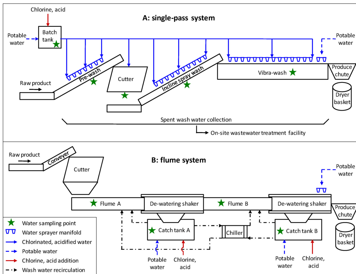
Fig. 1. Diagram of commercial fresh-cut produce washing processes, including a single-pass system (A) and flume system (B, modified from Luo et al., 2018). Water sampling points utilized during this study are also shown. In the flume system, wash water that was recirculated from flume A and B were kept in separate lines and did not mix in the chiller.
